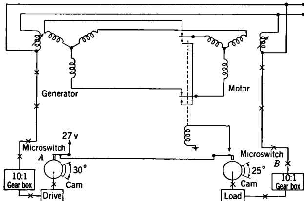
FIG. 16-8.—Microswitch phasing circuit.
